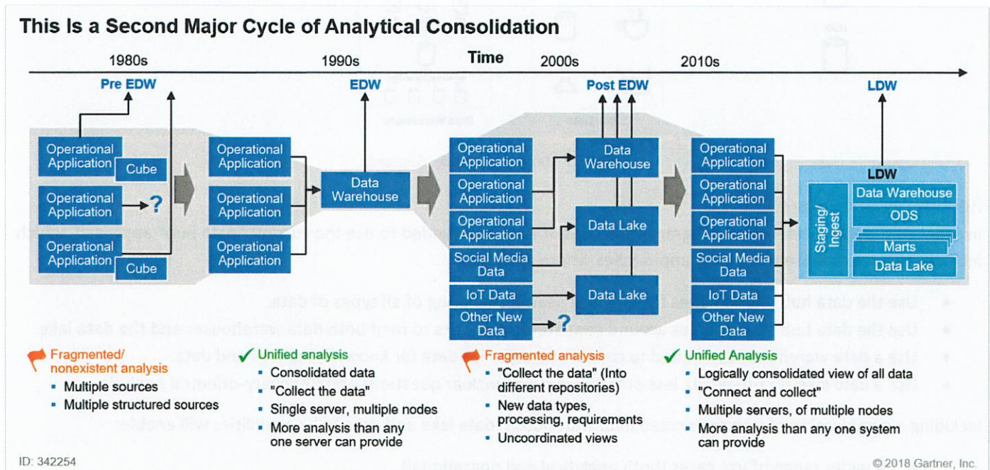
Figure 6 - Evolution of Logical Data Warehouse
