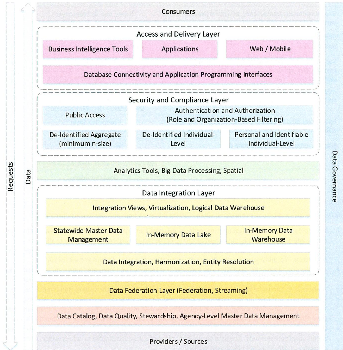
Figure 11 - Recommended Arkansas Data Hub Approach
