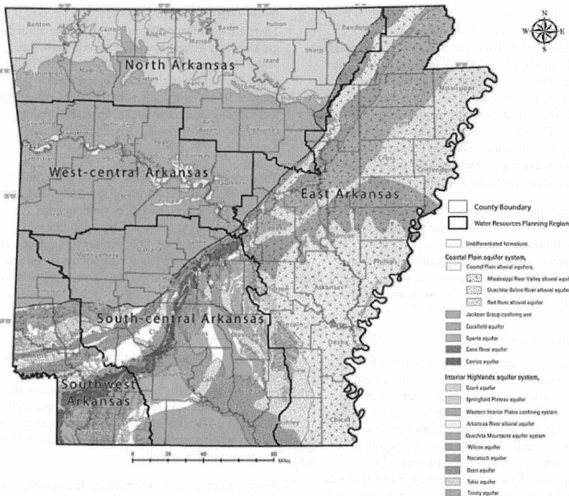
Figure 5-3. Aquifers of Arkansas
