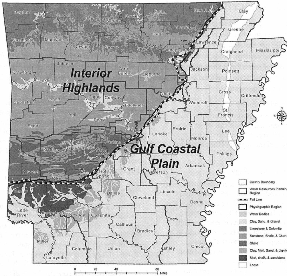
Figure 5-1. General Geology of Arkansas
